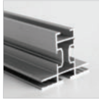
Profile / UYUP014101 Double Sided Maxi profile. King Frame Profile. 3 meters. 50x40 mm. Profil / UYUP014101 Double Sided Maxi Profil. King Frame Profil. 3 meter. 50x40 mm.
